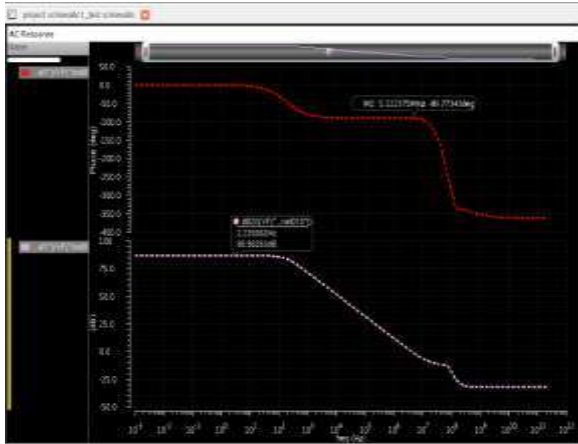
Fig 5: AC analysis of the schematic
