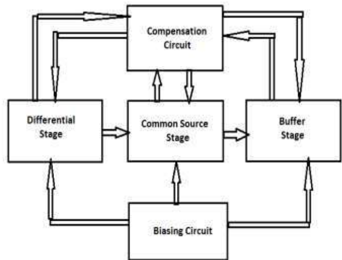
Fig. 1 shows block diagram of operational amplifier.
